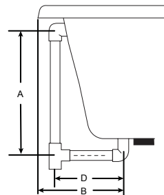
Drain/Overflow
