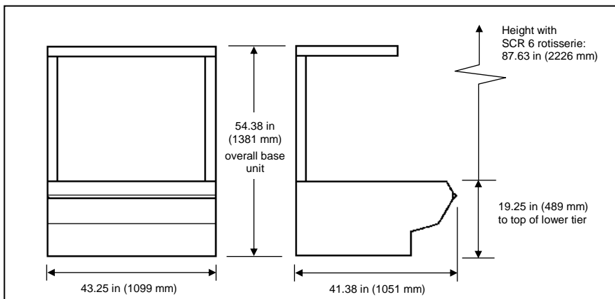
RMB 363 rotisserie merchandising base shown with SCR 6 rotisserie and HMR 103 self-serve merchandiser
